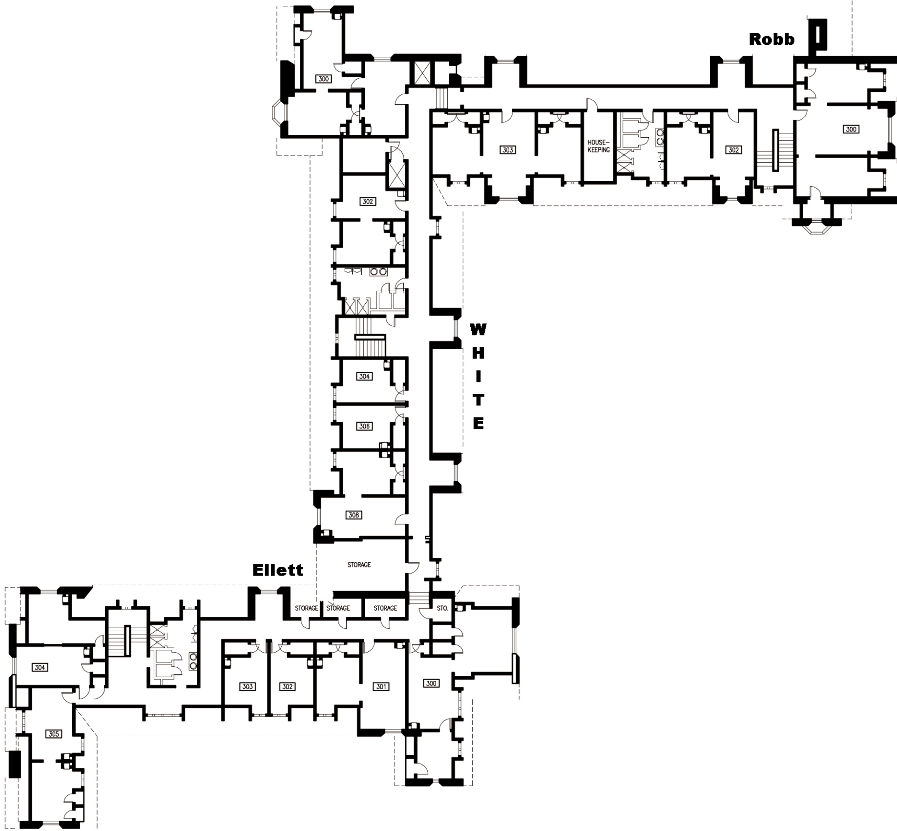
Robb, White, Ellett 3rd Floor 1/8"=1'-0"
