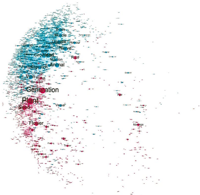
Fig. 7. Communities 3 and 8
